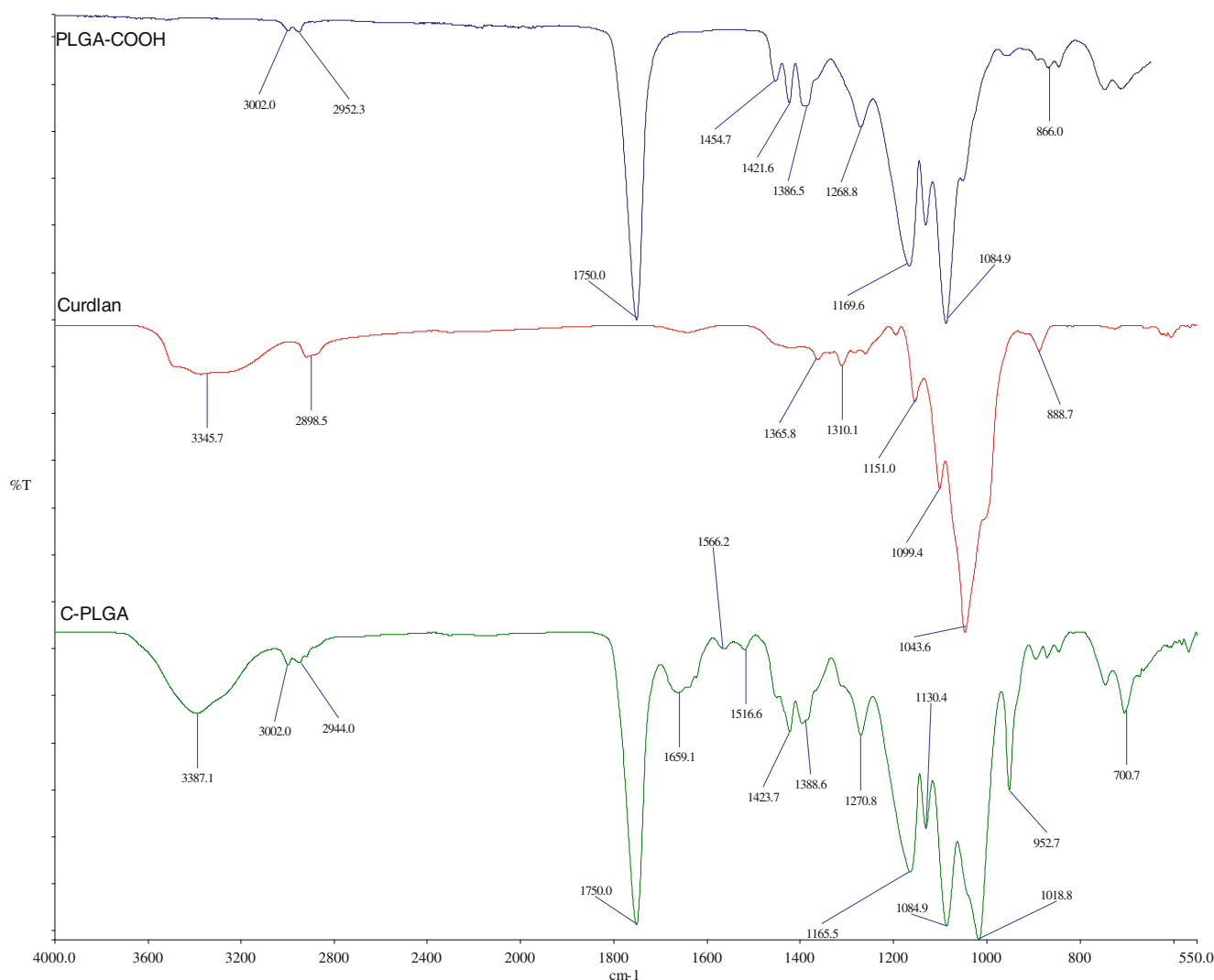
Fig. 4 FT-IR spectra of acid terminated PLGA-COOH, curdlan and Curdlan-PLGA copolymer.
